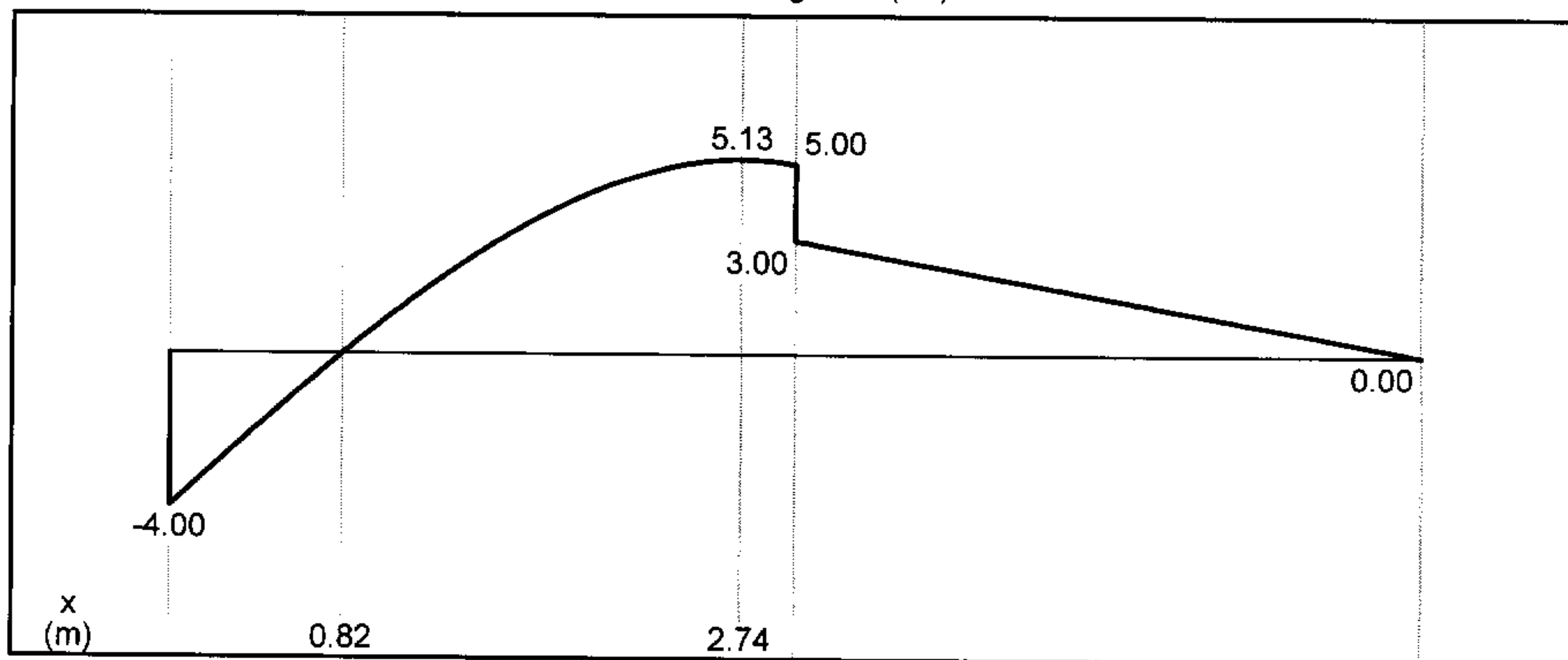
Moment Diagram (kN-m)
