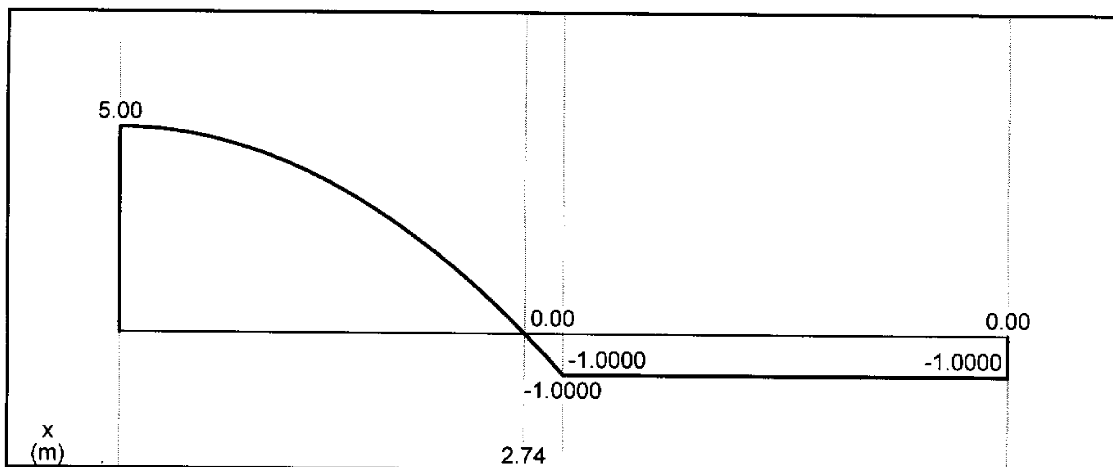
Shear Diagram (kN)
