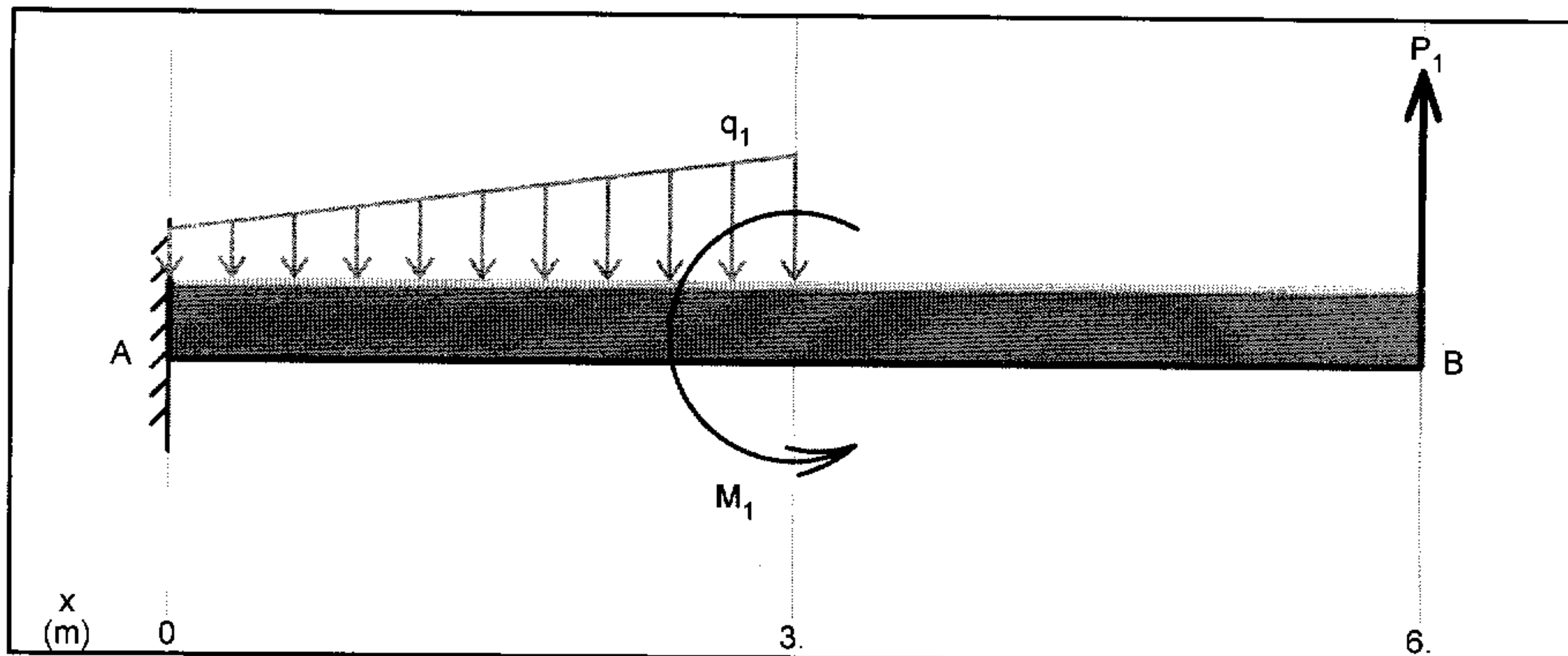
Load Diagram
