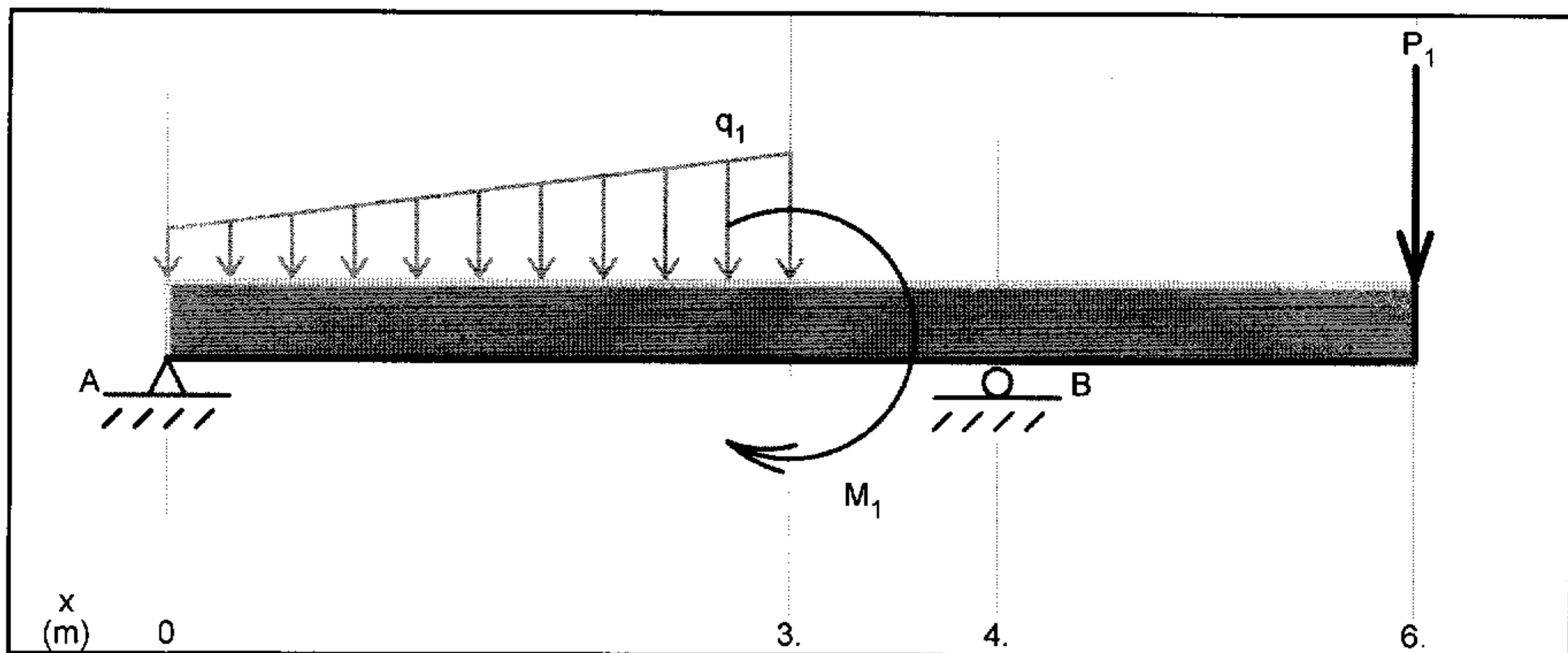
Load Diagram
