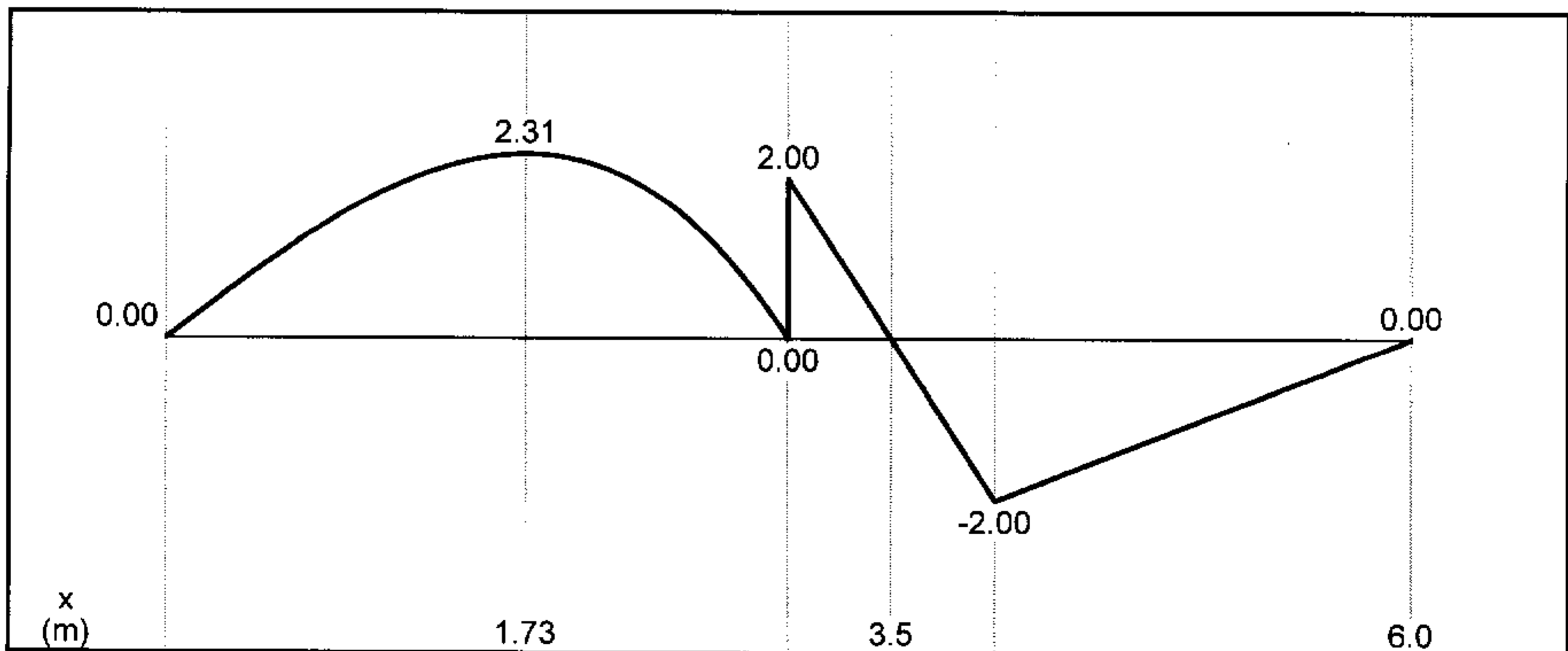
Moment Diagram (kN-m)
