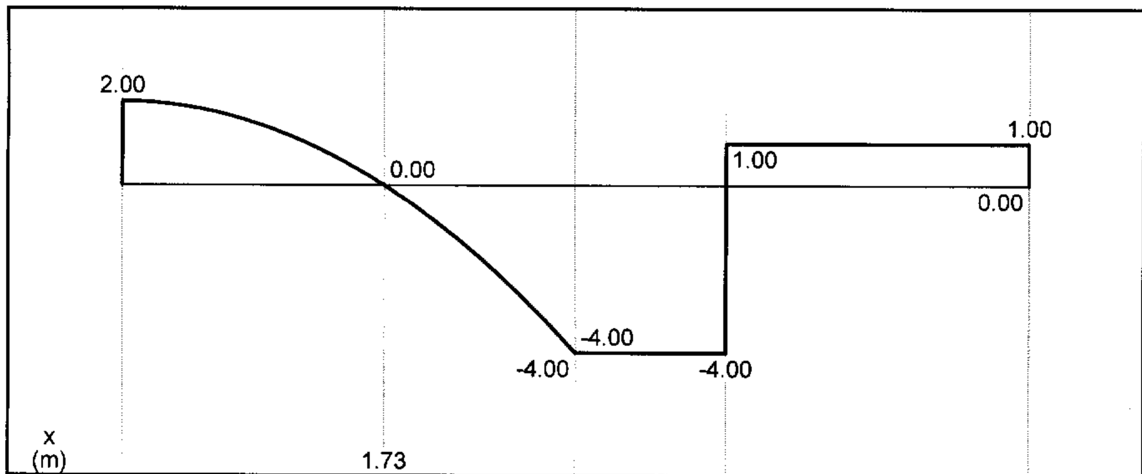
Shear Diagram (kN)
